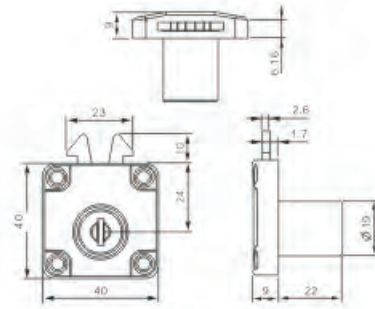
CYLINDER: D19mm*L22mm MATERIAL: ZINC ALLOY
