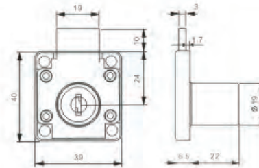
CYLINDER: D19mm*L22mm FINISH MATERIAL: TOTAL IRON NICKEL CHROME BLACK
