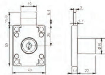
CYLINDER: D19mm*L22mm FINISH MATERIAL: TOTAL IRON NICKEL CHROME
