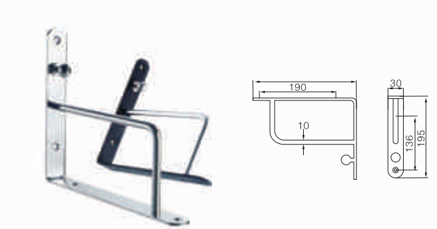
FJD-07-A03 RONDO-LINE SHELF WARDROBE BRACKETS COLOR: CHROME/NICKEL/ GOLD/ BLACK PLATED WEIGHT CAPACITY: 40KG
