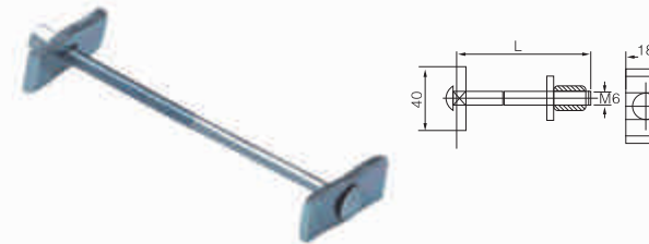
FJD-04-026 CONNECTTING BOLT LENGTH: 65-150MM MATERIAL: STEEL FINISH: ZINC PLATED
