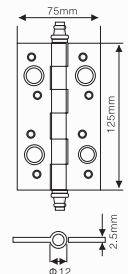
FJD-35-007 STEEL HINGE
