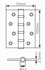
FJD-35-006 STEEL HINGE
