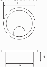
FJD-46-58002 SIZE: M=Φ80/60 B:20/12 H: 88/66 MATERIAL: ZINC ALLOY FINISH: CHROME/BRUSH NICKEL/POLISH/ANTIQUE BRASS
