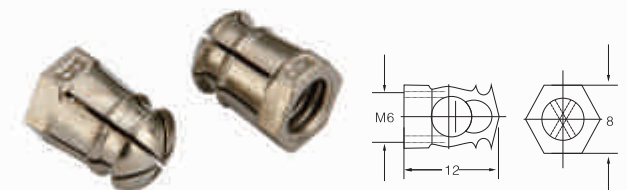
FJD-04-029 EXPANDING NUT SIZE: SEE DRAWING FINISH: NICKEL PLATED
