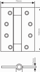
FJD-35-005 STEEL HINGE
