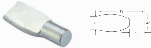
FJD-03-017 SHELF SUPPORT SIZE:M5x19 FINISH: ZINC/NICKEL PLATED
