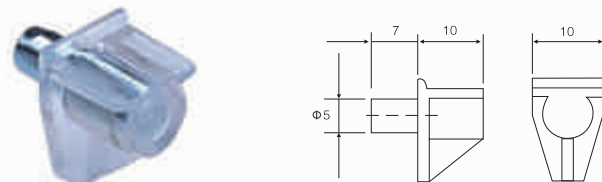
FJD-03-018 SHELF SUPPORT SIZE:M5x17 PLASTIC PART COLOR:CLEAR/BROWN/WHITE/BLACK FINISH:ZINC/NICKEL PLATED
