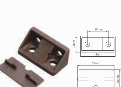
FJD-08-CJ3920A PLASTIC CONNECTOR WITH COVER
