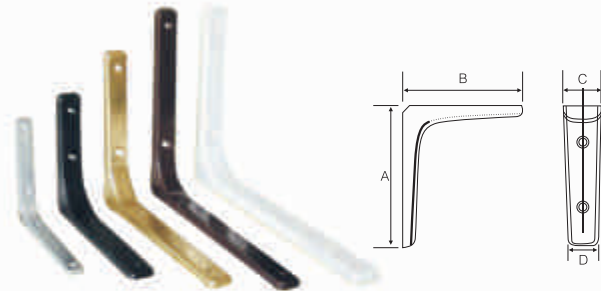
FJD-07-120 SIZE: 30x30--400x300MM THICKNESS: 1.2--2.0MM MAX CARRYING CAPABILITY: 18KG--50KG FINISH: WHITE/BROWN/ GREY/BLACK, ETC.
