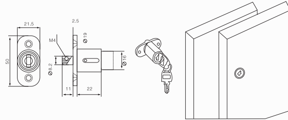
A set diagram Installation diagram
