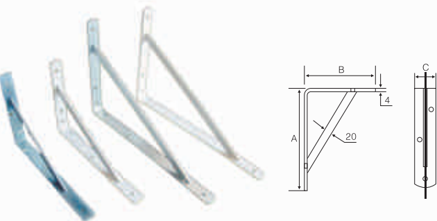
FJD-07-201 SIZE: 200x300, 250x400, 330x500MM MAX CARRYING CAPABILITY: 200KG--300KG FINISH: ZINC PLATED/COLOR PAINTING
