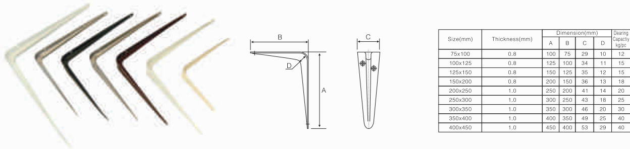
FJD-07-001 TRIANGLE BRACKET COLOR: WHITE/BROWN/GRAY/BLACK
