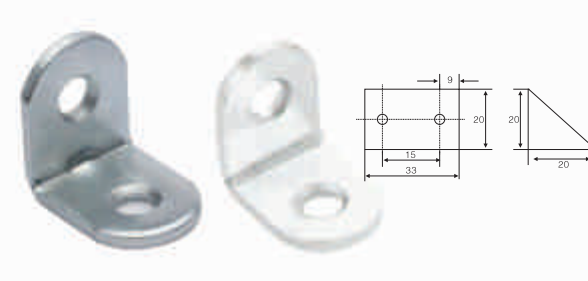
FJD-08-03 MATERIAL: STEEL FINISH: ZINC PLATED SIZE: 20x20x15MM
