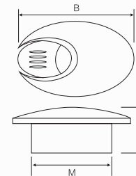
FJD-46-58001 SIZE: M=Φ80/60 B:88/66 H: 20/12 MATERIAL: ZINC ALLOY FINISH: CHROME/BRUSH NICKEL/POLISH/ANTIQUE BRASS
