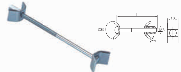
FJD-04-027 CONNECTTING BOLT LENGTH: 65-150MM MATERIAL: STEEL FINISH: ZINC PLATED
