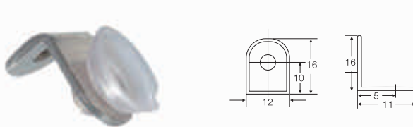
FJD-03-020 SHELF SUPPORT SIZE: SEE DRAWING FINISH:ZINC/NICKEL PLATED
