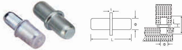
FJD-03-016 SHELF SUPPORT SIZE:M3x16,M5x16, M6x18, M8x20 FINISH:ZINC/NICKEL PLATED
