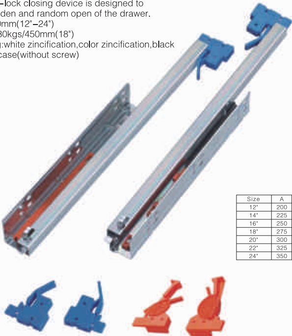
Non-adjustable high&low slide rail lock Adjustable high slide rail lock
