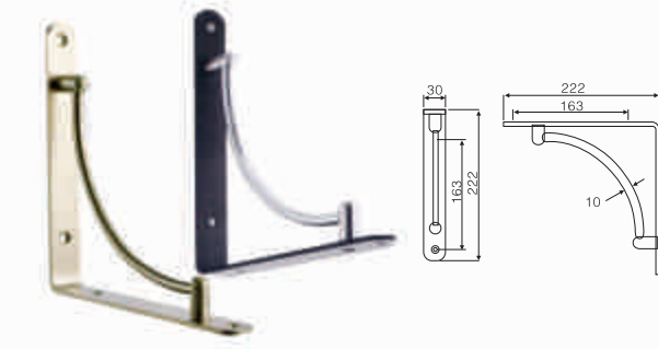
FJD-07-A02 C TYPE BRACKET COLOR: CHROME/NICKEL/ GOLD/ BLACK PLATED CARRYING CAPABILITY: 20KG
