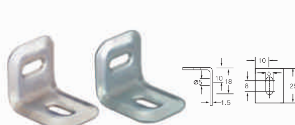
FJD-08-50023 MATERIAL: STEEL FINISH: ZINC PLATED
