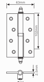
FJD-35-008 STEEL HINGE
